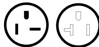
NEMA 5-20R NEMA 5-20P
